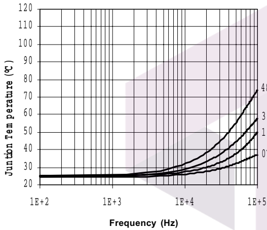
Figure 7. IR2133J Junction Temperature vs Frequency Driving (IRGPC20KD2) Rgate = 5.1Ω @ Vcc = 15V
