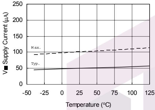
Figure 28A. V_{BS} Supply Current vs. Temperature
